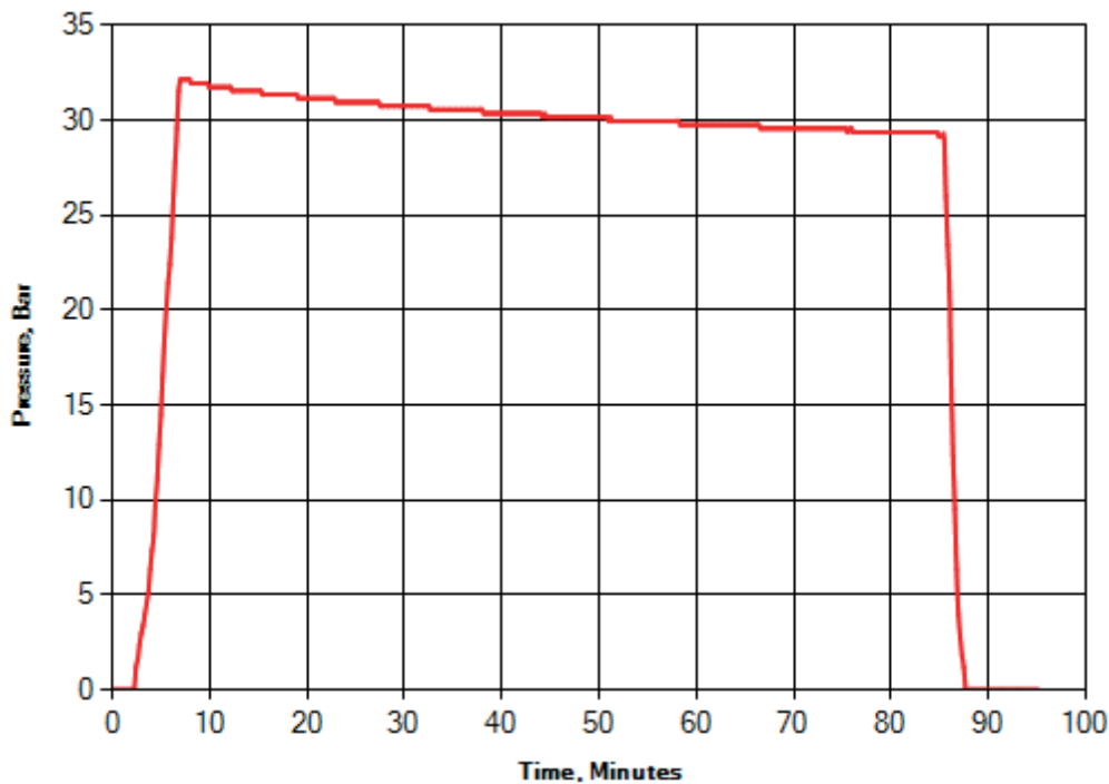
Pressure graph
